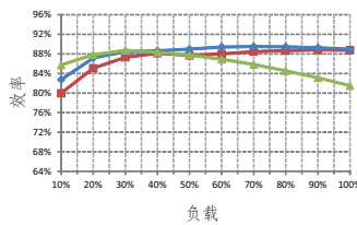
RSD-60G-5
