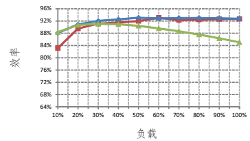
RSD-60G-12
