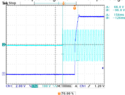
INPUT=115VAC/50HZ @ FULL LOAD
