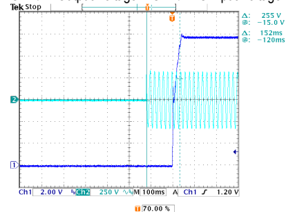
INPUT=230VAC/50HZ @ FULL LOAD
